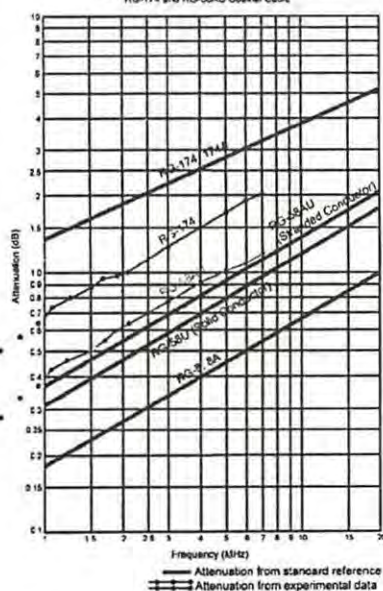
Attenuation Per Hundred Feet RG-174 and RG-58AU Coaxial Cable
