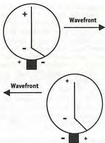
Figure 2: Combining a vertical antenna with a loop eliminates the 180 degree ambiguity of the ordinary loop.
