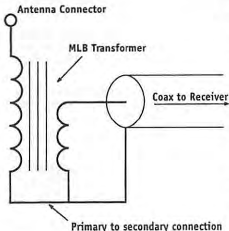
Figure 2. A conventional MLB has a connection that forces the shield of the coax to act as a part of the antenna. More noise pickup is the result.
