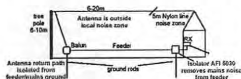
Figure 3. This long-wire antenna design keeps all active parts of the antenna away from noise sources and shunts noise on the house grounding system to earth.
