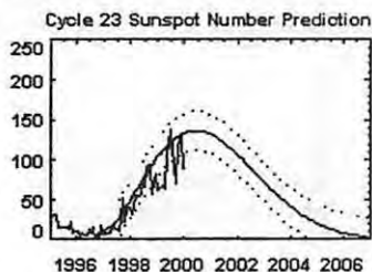
Figure 1 Solar Cycle 23 is not measuring up to previous predictions.
