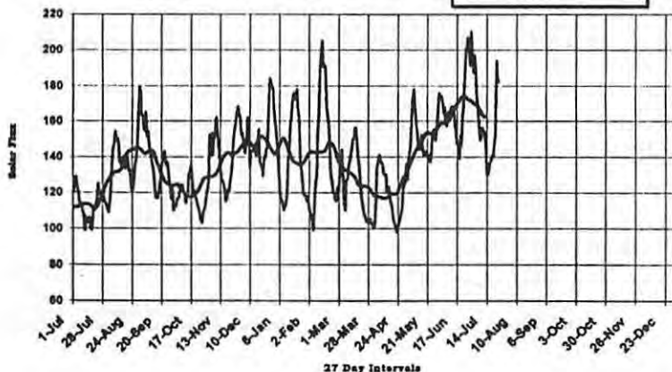
Solar Flux: 27-Day Moving Average: 1998-1999
