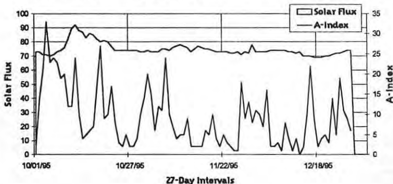
SOLAR FLUX & A-INDEX: OCT-DEC '95
