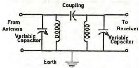
Figure 1: A resonant preselector provides front end selectivity and a static discharge path to ground to protect your expensive receiver. Its loss is greater than the Transmatch.
