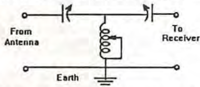
Figure 2: The Transmatch antenna coupler acts as a high pass filter providing inferior selectivity compared to the resonant preselector. It is more efficient, however.
