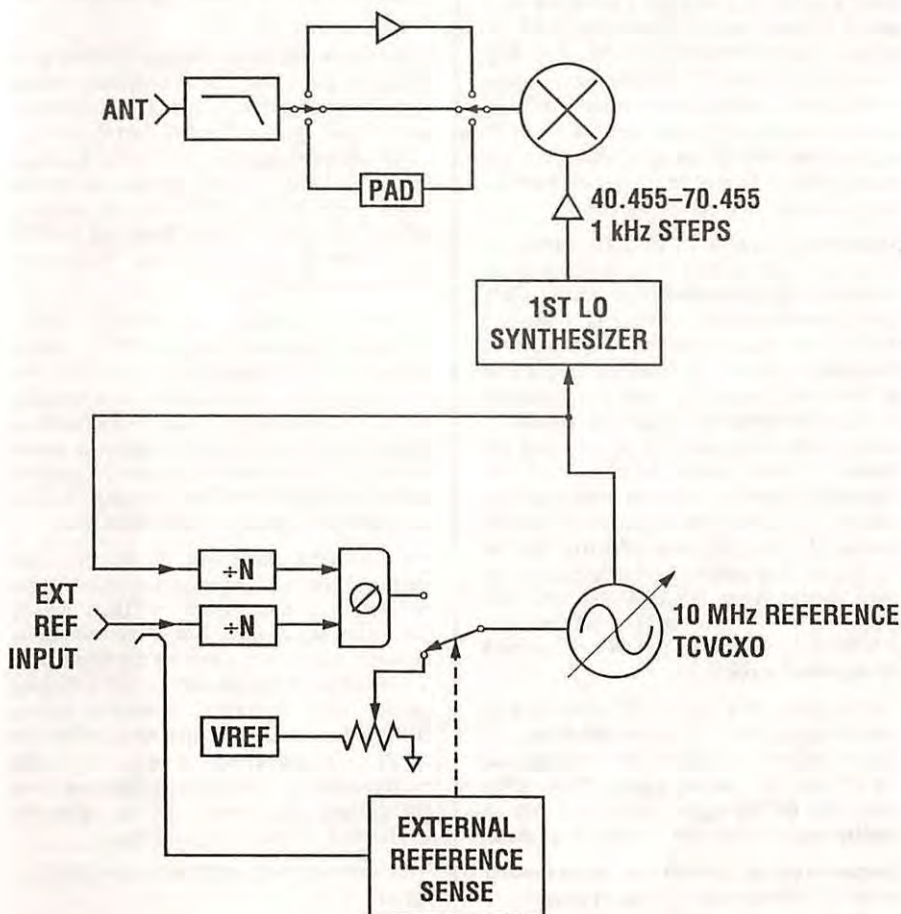
Figure 3. The local oscillator synthesizer permits selection of the receive frequency to an accuracy determined by a precision reference frequency.
