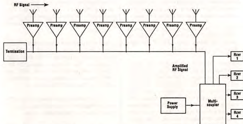
Figure 2 Hermes Loop Array schematic illustrates antenna operation
