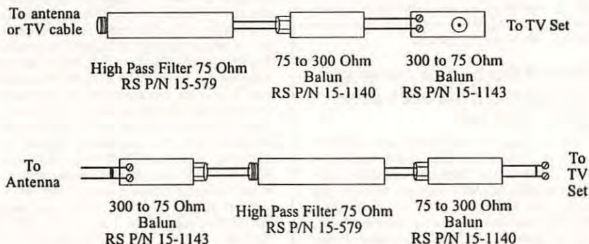
Figure 1. Breaking the common mode current path for 75 and 300 ohm TV antenna systems
