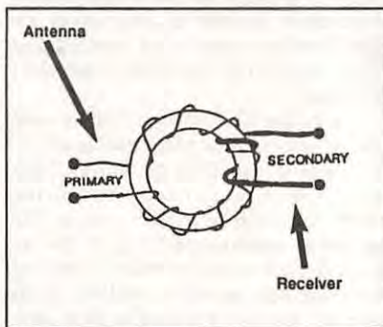
Figure 1. Ferrite toroidal core wound as a step-down transformer. Hall-Patch & Bryant, "Impedance Matching a Beverage Antenna to a Receiver, Proceedings 1988 ."
