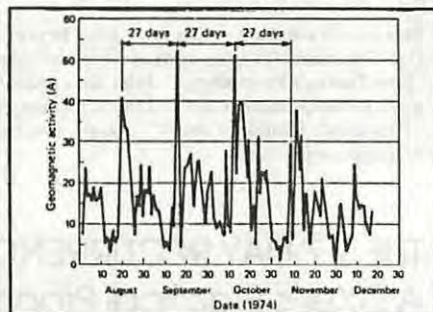
Figure 2- Geomagnetic activity (A Index) as a function of time (Aug. 1 through Dec. 17, 1974). Note approximate 27-day recurrence tendency of values. (from Jacobs)
