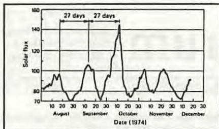
Figure 1 - Solar flux as a function of time (Aug. 1 through Dec. 17, 1974). Note tendency towards approximate 27-day recurrence. (from Jacobs)
