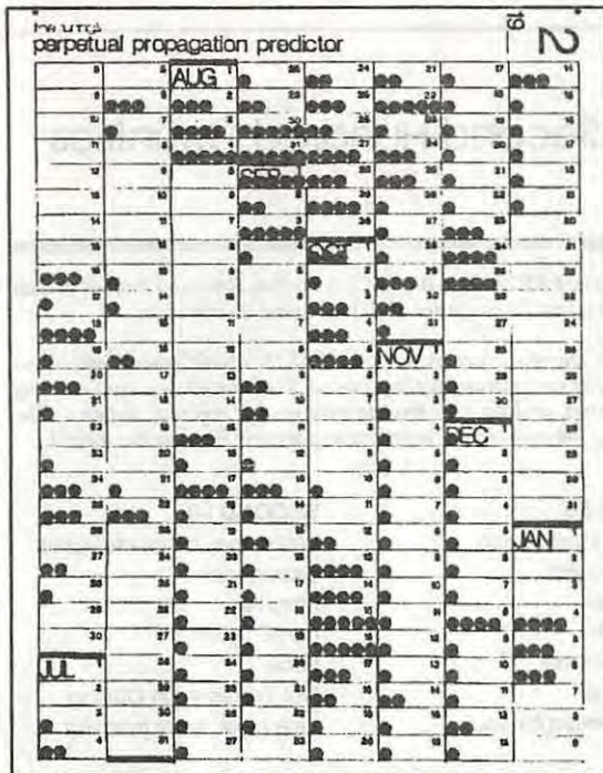
Figure 3 - Fine Tuning's 27-day Perpetual Propagation
