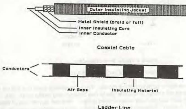
Figure 2. Coax and Ladder Line
