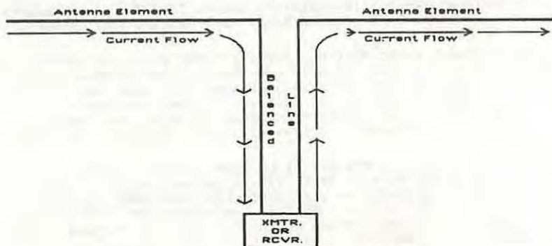
Figure 1. Antenna/Feedline Current Flow
