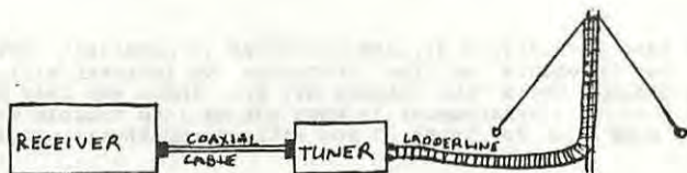
FIGURE 4 TUNED INVERTED V MULTI-BAND ANTENNA
