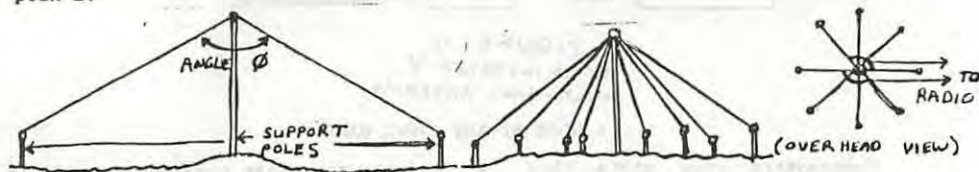
FIGURE 3 "GANDED" INVERTED V'S
