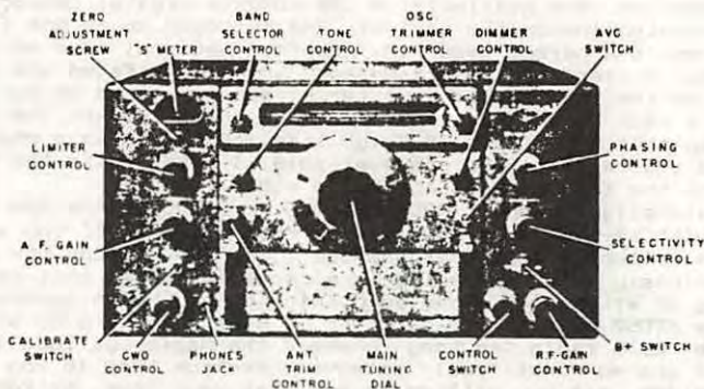
Figure No. 5. Front view of Receiver
