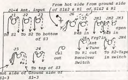
Figure 5: Back panel wiring.
