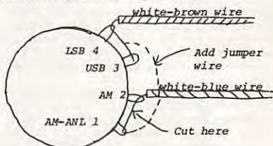
REAR VIEW OF MODE SWITCH SHOWING SELECTIVITY MODIFICATIONS
