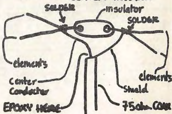
Fig. 2. DETAIL OF THE CENTER INSULATOR
