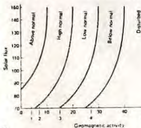
Fig. 1 - Interaction of given values of solar flux and geomagnetic activity determine expected h.f. ionospheric propagation conditions. (Example: S.F.=80, Ap=25 expect BELOW NORMAL conditions.) From mid-1974 to mid-1976, conditions recurred 27 days later exactly as defined in the above categories 63% of the time, and within an accuracy of one category 82% of the time (counting differences between LOW and BELOW NORMAL as a miss.)
