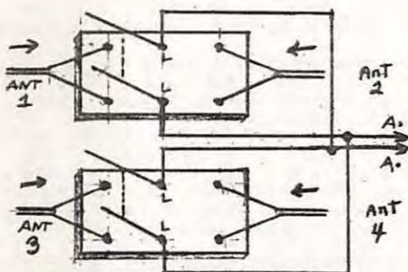
Diagram Above, Photo Below, 2 Leviton #9919 Double-Knife Switches Connecting 4 Dipoles
