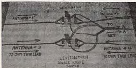
Diagram Above, Photo Below, 2 Leviton #9919 Double-Knife Switches Connecting 4 Dipoles
