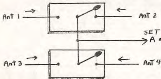
Two Leviton # 9914 single-knife switches connecting four longwires.
